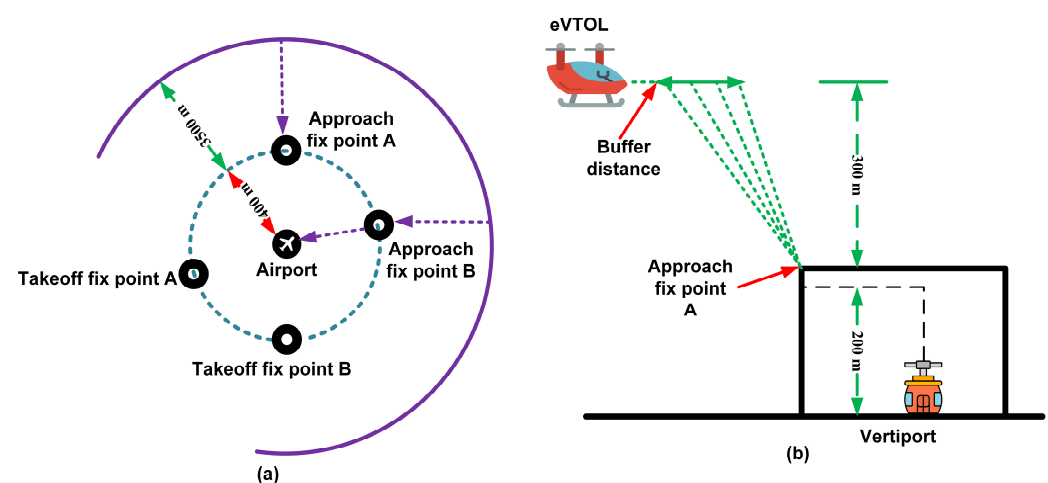
Figure 4. (a) Horizontal and (b) vertical landing approaches of eVTOL aircraft.
